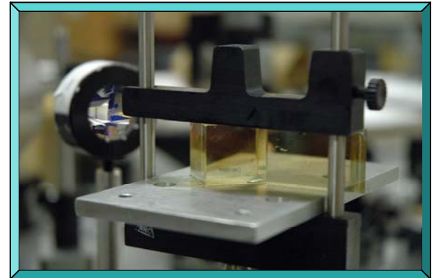
Surface plasmon resonance sensor
