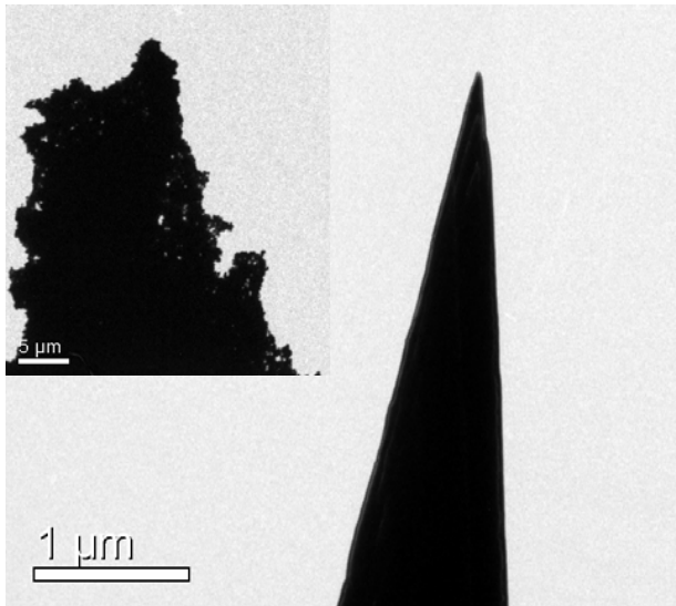
Significant improvement in Au STM tip sharpness and smoothness
