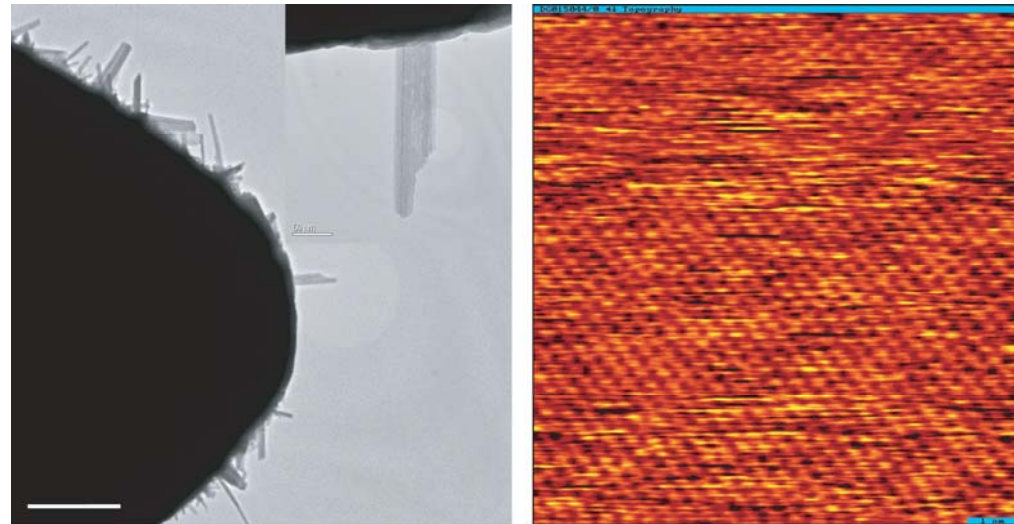
Left, TEM image of carbon nanotube STM tip following imaging of graphite. At right, STM image of graphite.
