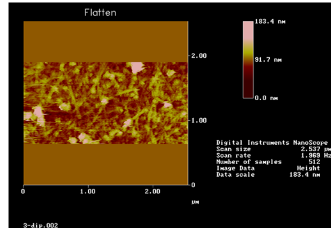
AFM image of CNT film after three dips
